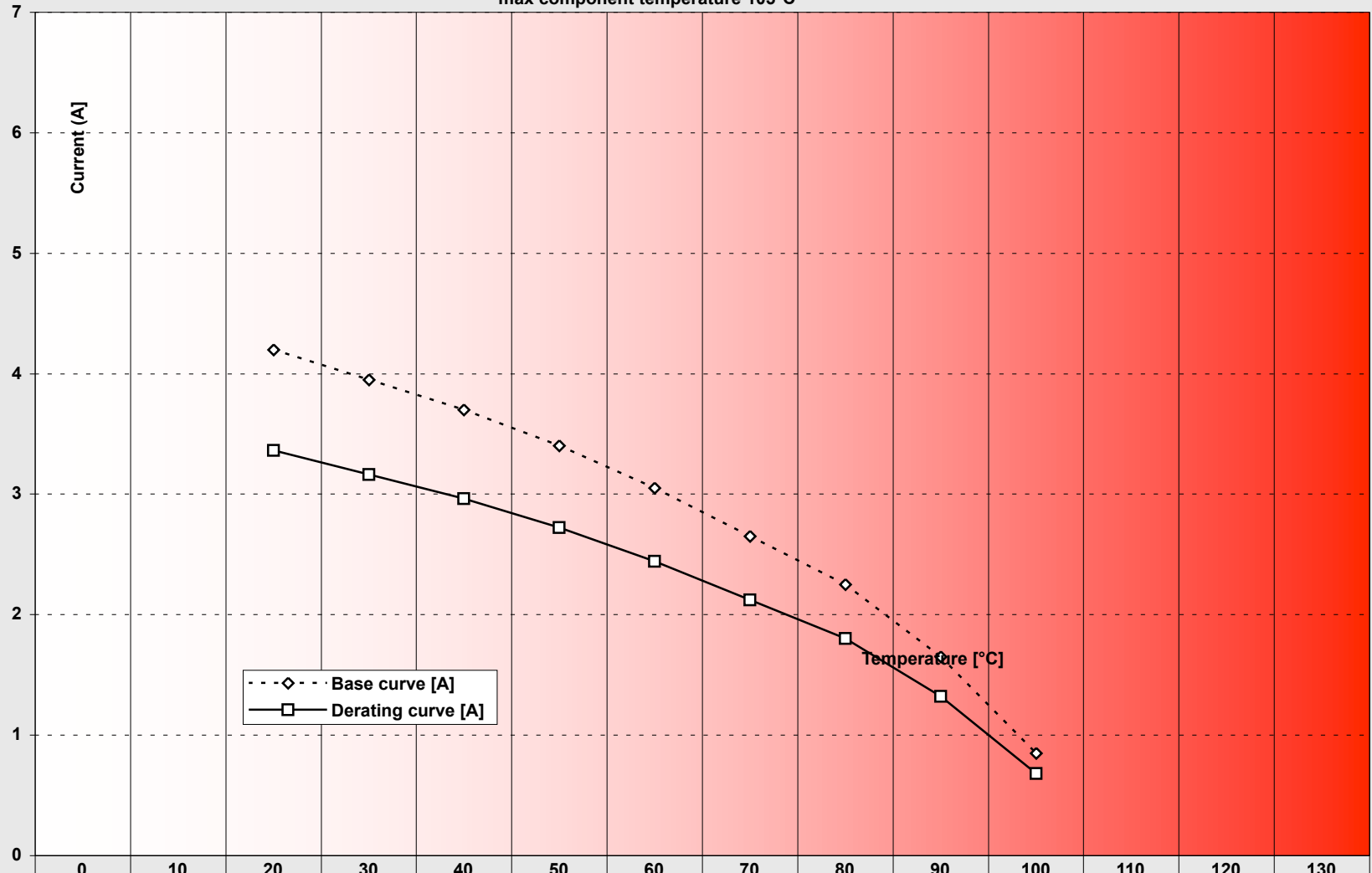
DERATING CURVE (Current carrying capacity acc. IEC 60512-5-2 Test 5b) MiniBridge A/P 8p with 250 mm stranded flat ribbon cable AWG 26 max component temperature 105°C
