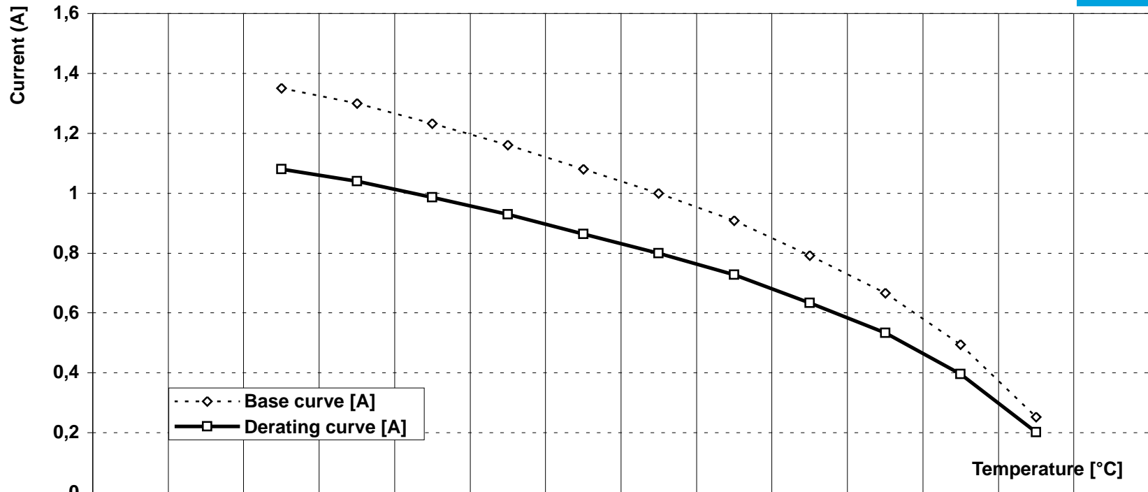
DERATING CURVE (Current carrying capacity acc. IEC 60512-5-2 Test 5b) Microspeed connector with 50 contacts
