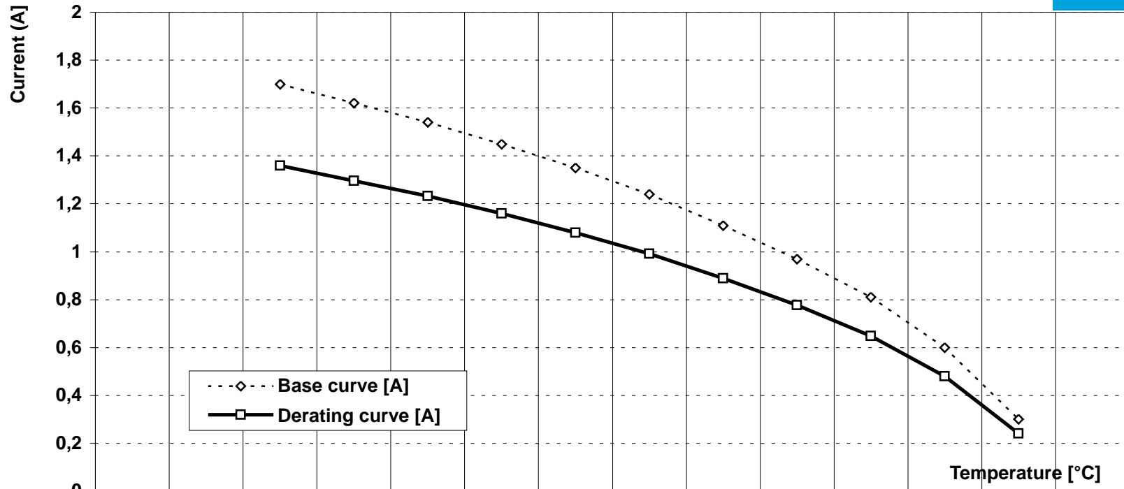
DERATING CURVE (Current carrying capacity acc. IEC 60512-2-5 Test 5b) ERmet connector module B with 125 contacts
