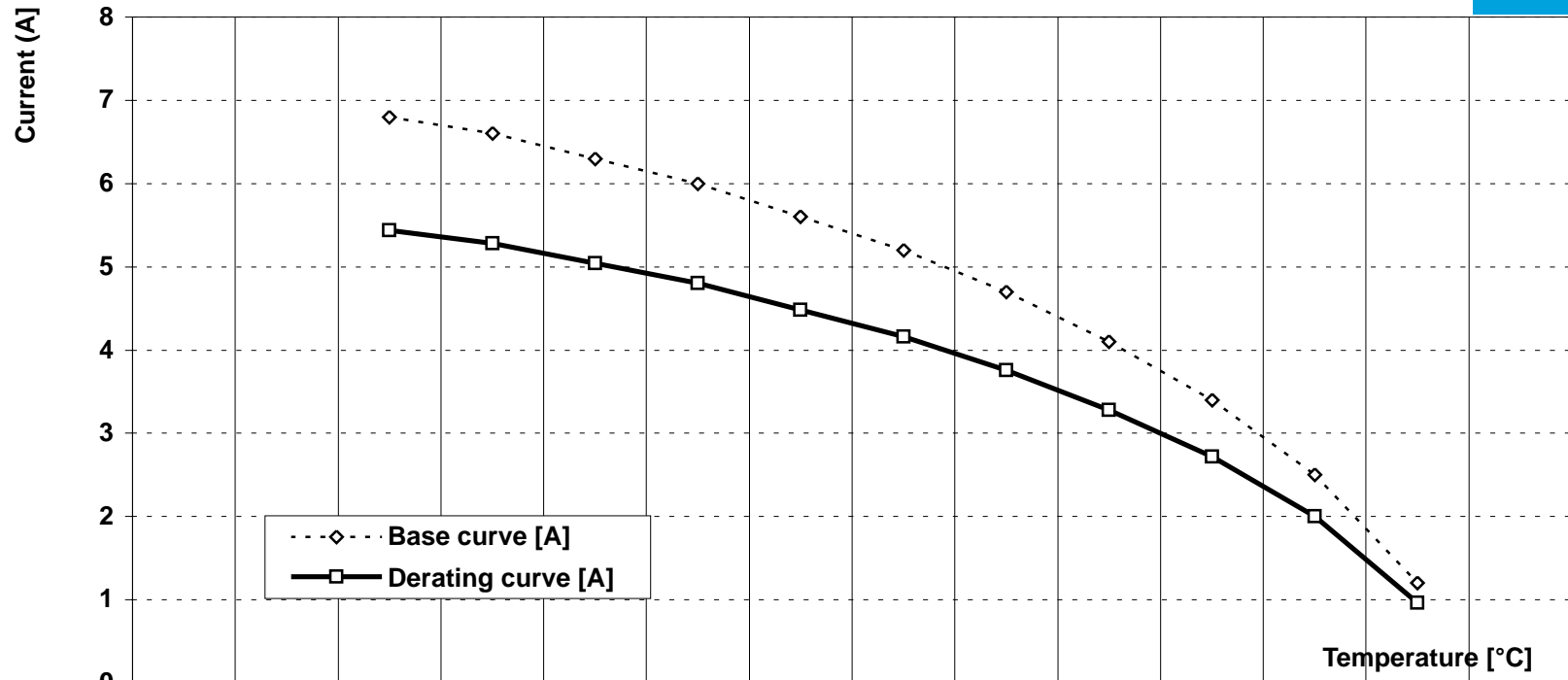
DERATING CURVE (Current carrying capacity acc. IEC 60512-5-2 Test 5b) IEC 60603-2 connector F48 with 48 contacts
