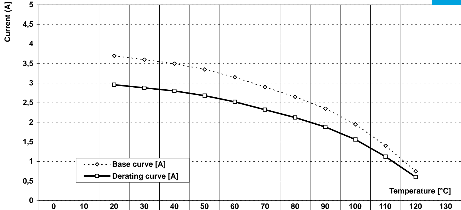
DERATING CURVE (Current carrying capacity acc. IEC 60512-5-2 Test 5b) IEC 60603-2 connector C/2 and R/2 with 48 contacts
