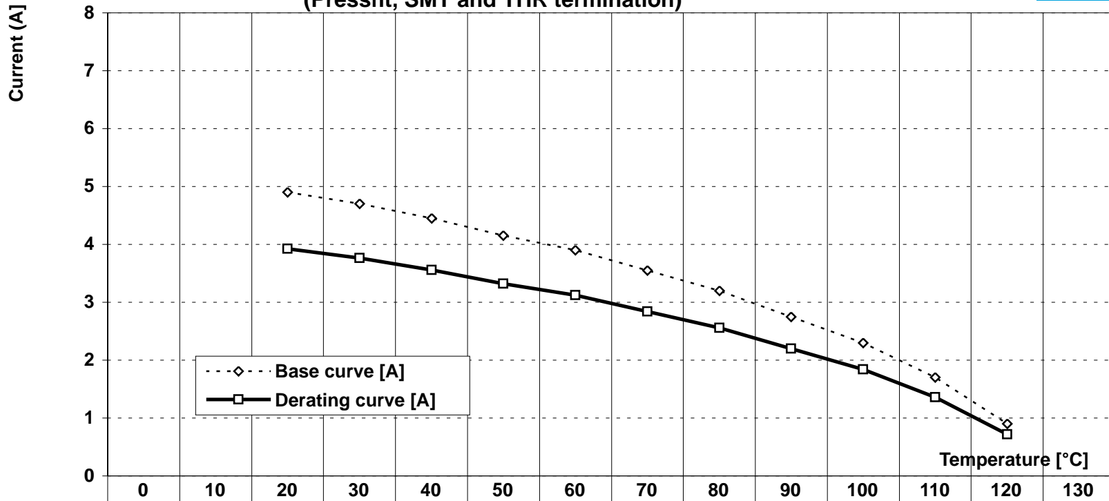
DERATING CURVE (Current carrying capacity acc. IEC 60512-5-2 Test 5b) D-Sub connector TMC 90° and 180° Ba 8 with 37 contacts (Pressfit, SMT and THR termination)
