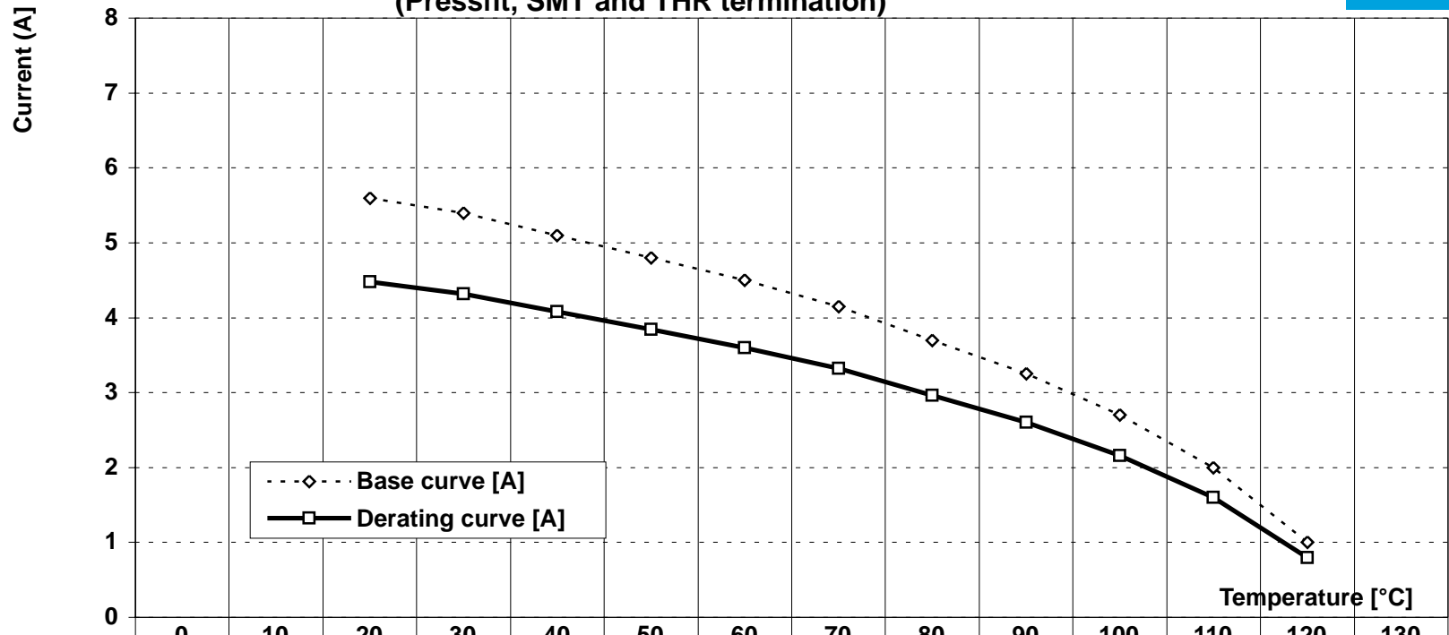
DERATING CURVE (Current carrying capacity acc. IEC 60512-5-2 Test 5b) D-Sub connector TMC 90° and 180° Ba 8 with 25 contacts (Pressfit, SMT and THR termination)
