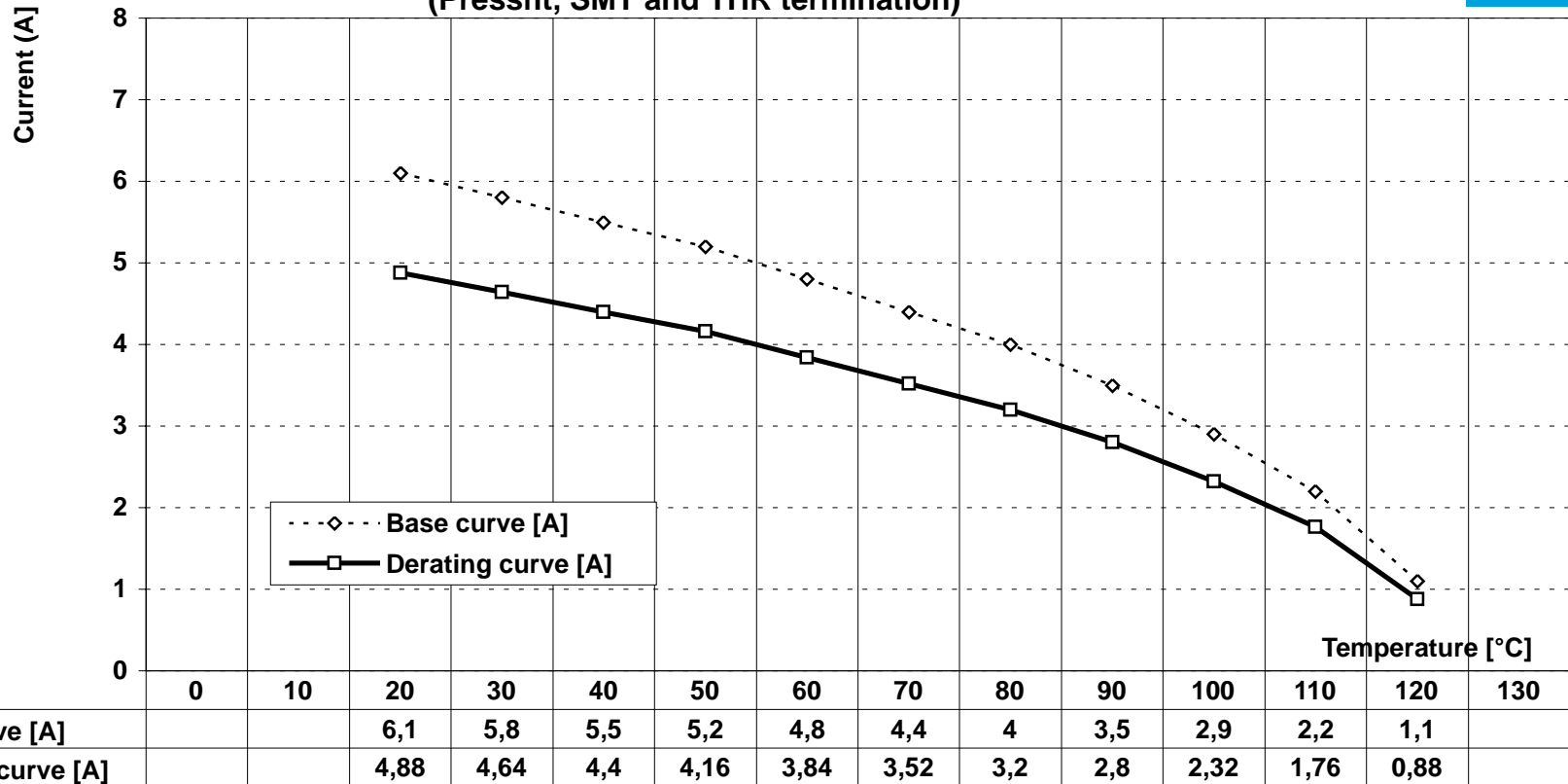
DERATING CURVE (Current carrying capacity acc. IEC 60512-5-2 Test 5b) D-Sub connector TMC 90° and 180° Ba 8 with 15 contacts (Pressfit, SMT and THR termination)
