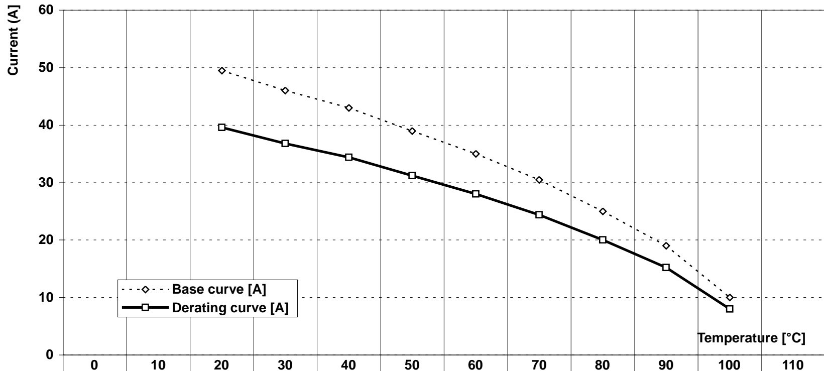
DERATING CURVE (Current carrying capacity acc. IEC 60512-5-2 Test 5b) Power Tap connector (SVA) with formed thread 6 contacts (pressfit termination)
